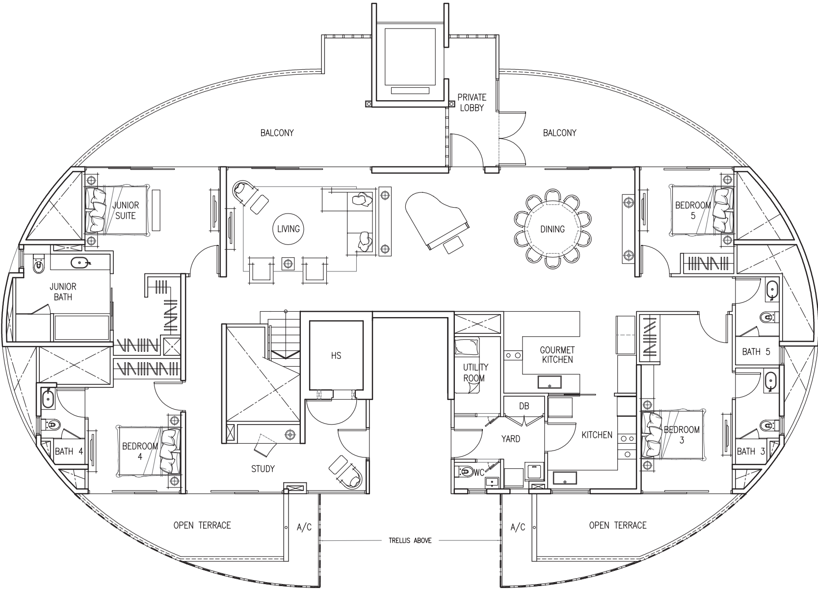
Lower Level
