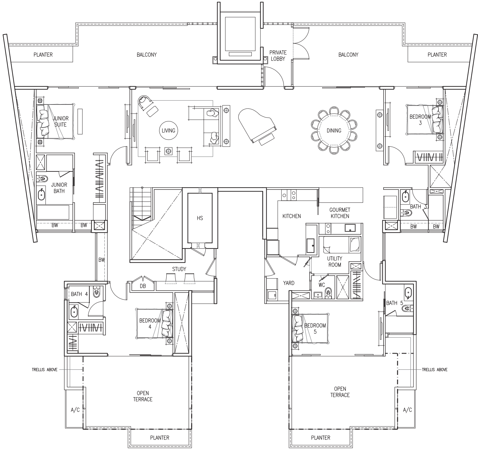
Lower Level
