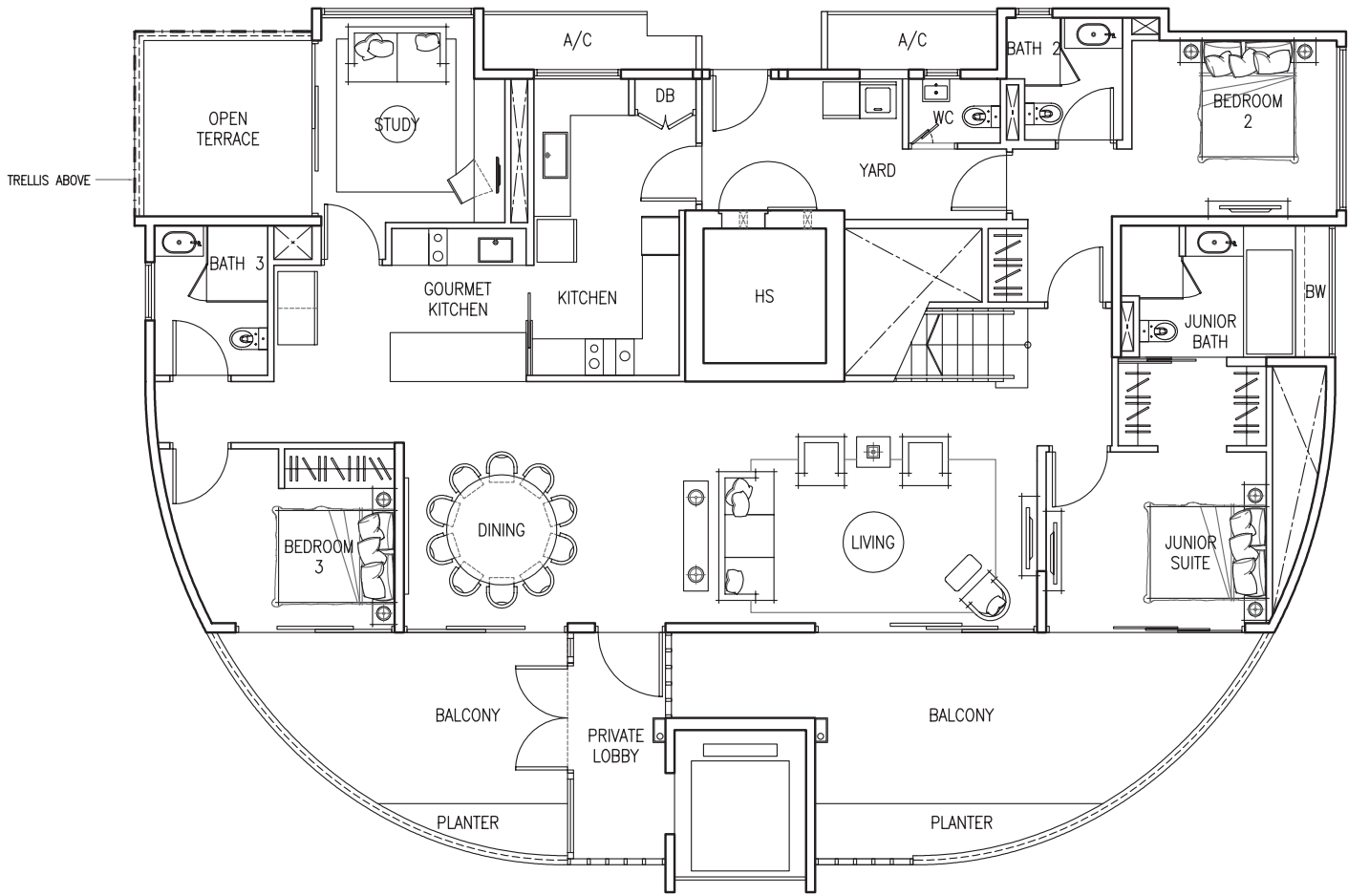
Lower Level
